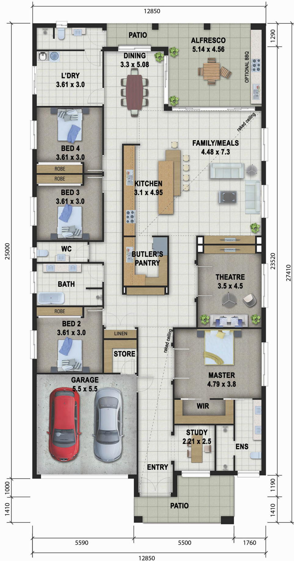
FLOOR PLAN ROSEDALE OPTION 1
